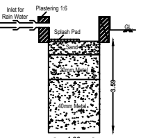
RAIN WATER PERCOLATION PIT
