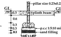
FOUNDATION DETAILS
