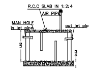
SEPTIC TANK SECTION
