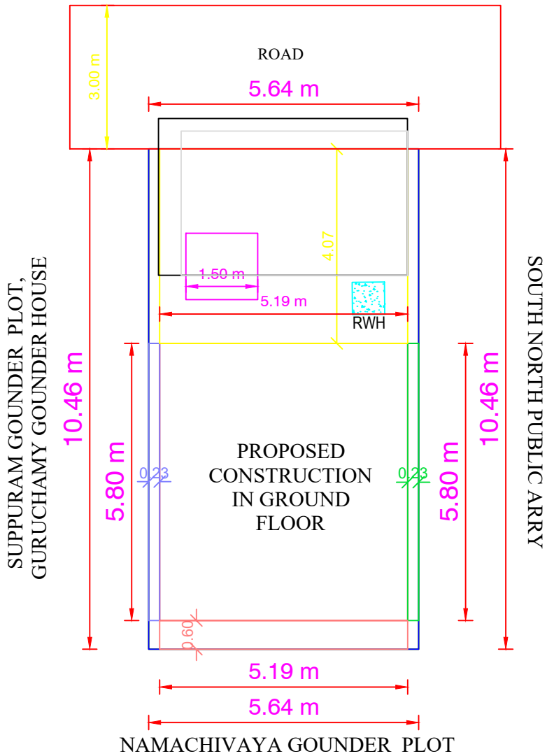
SITE PLAN
