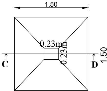
SECTION - 'CD'
