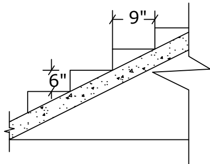
Staircase Detail Not To Scale
