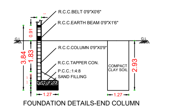
FOUNDATION DETAILS-END COLUMN
