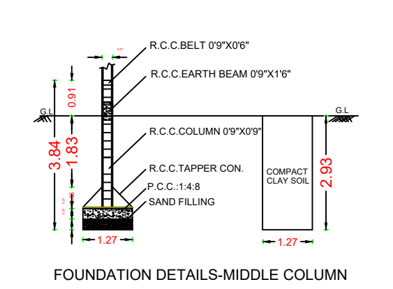
FOUNDATION DETAILS-MIDDLE COLUMN
