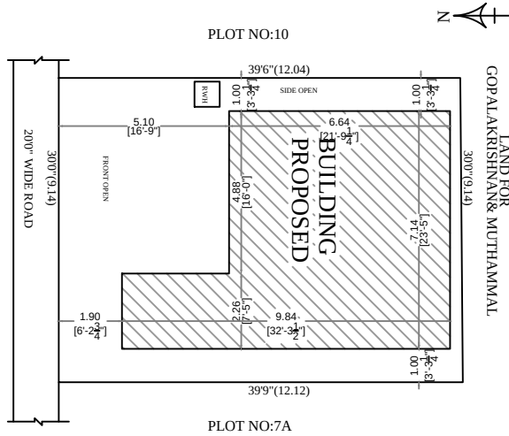
SITE PLAN
