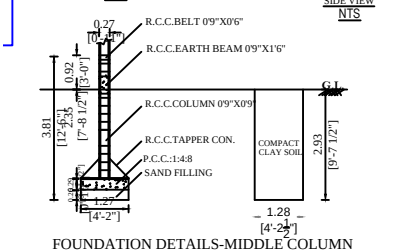
FOUNDATION DETAILS-MIDDLE COLUMN NTS
