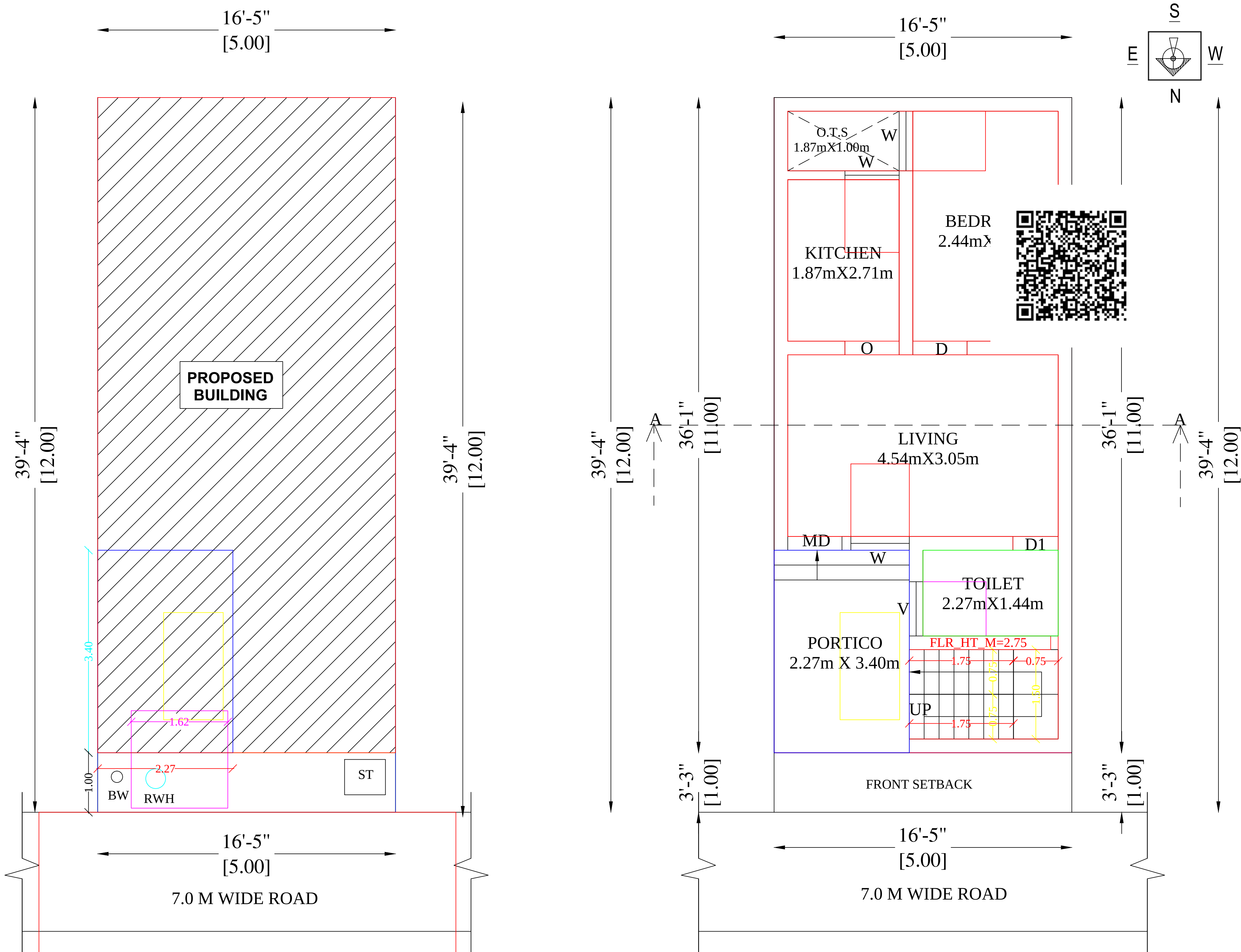
SITE PLAN
