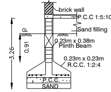
FOUNDATION DETAILS
