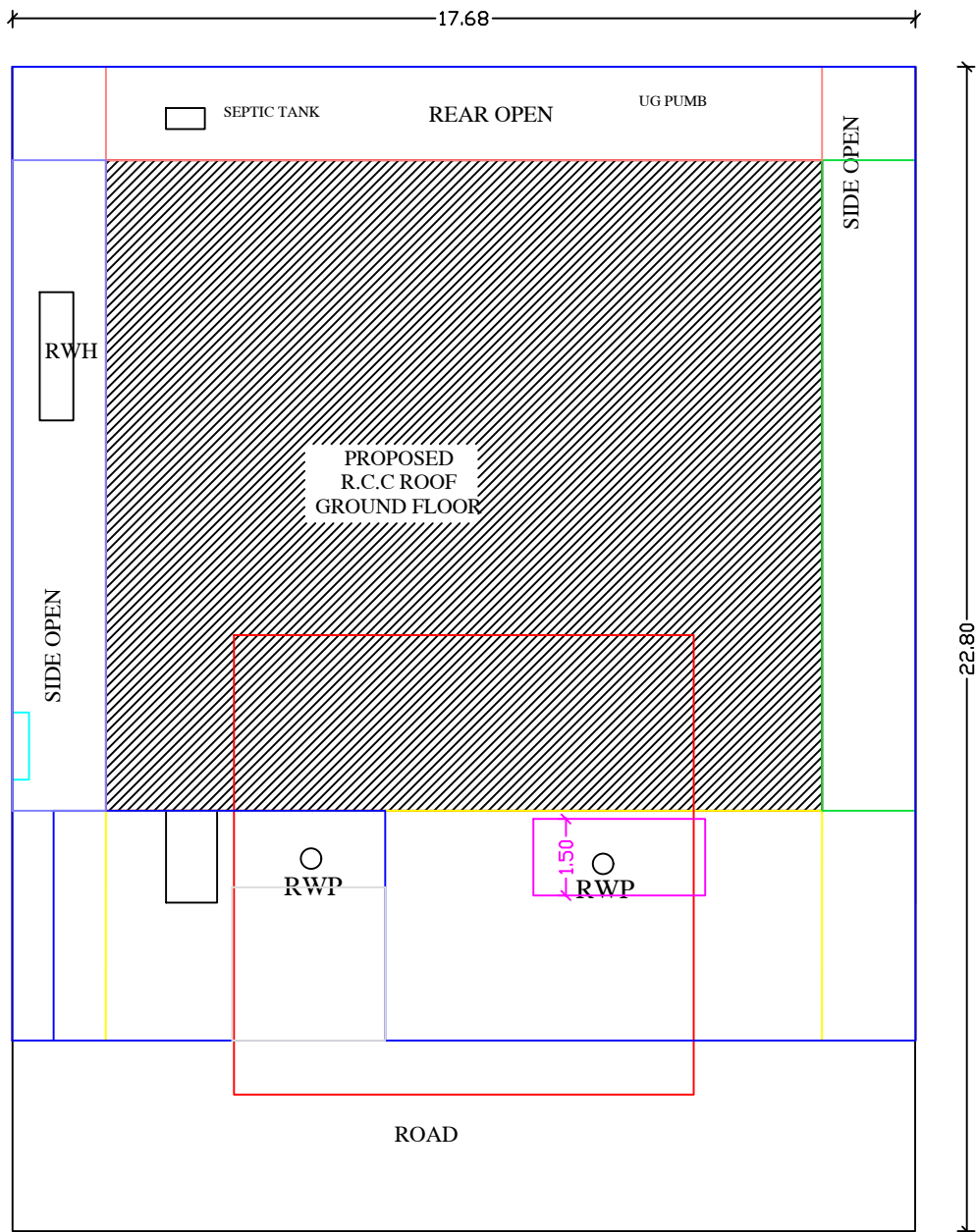
SITE PLAN
