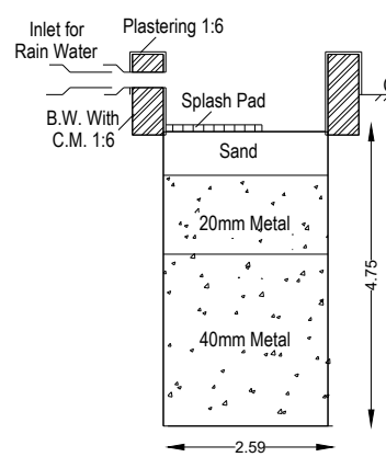
RAIN WATER PERCOLATION PIT
