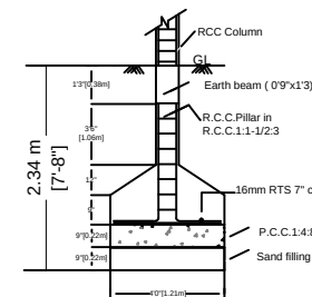
FOUNDATION DETAILS
