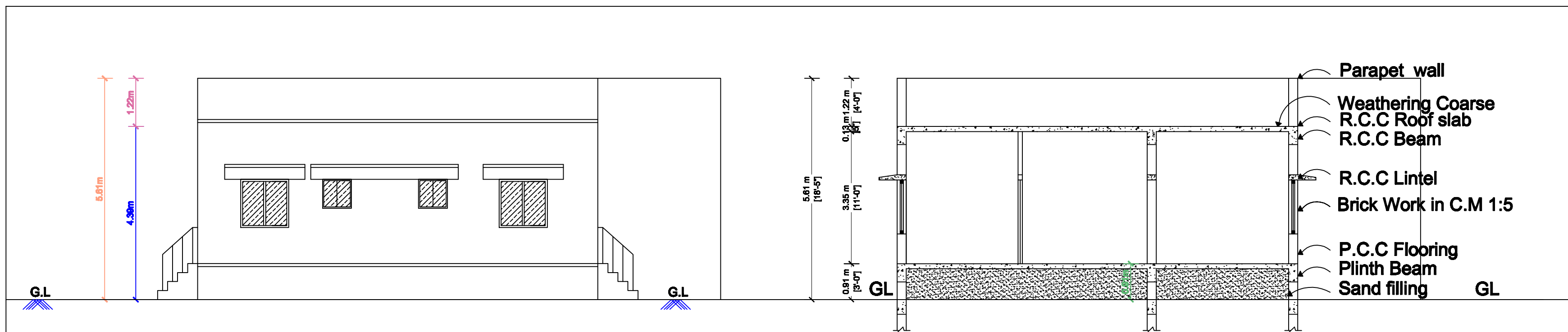
FRONT ELEVATION
