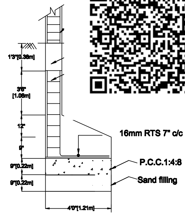
FOUNDATION DETAILS
