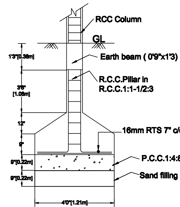
FOUNDATION DETAILS
