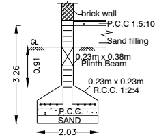
FOUNDATION DETAILS
