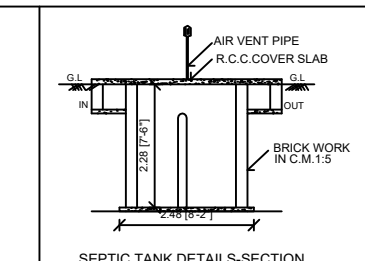
SEPTIC TANK DETAILS-SECTION
