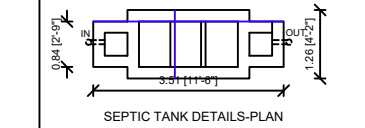
SEPTIC TANK DETAILS-PLAN
