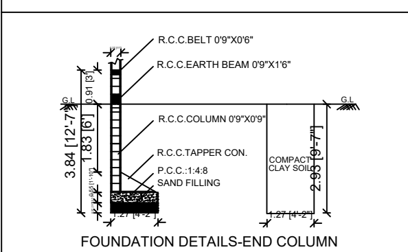
FOUNDATION DETAILS-END COLUMN
