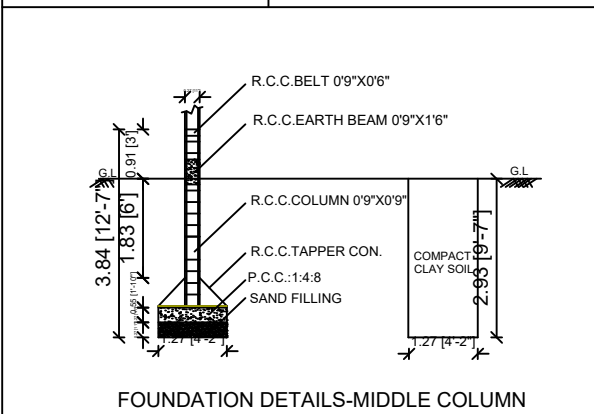
FOUNDATION DETAILS-MIDDLE COLUMN
