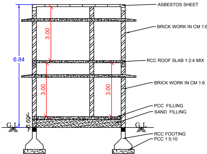
SECTION AB
