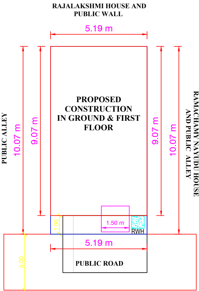
SITE PLAN
