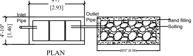
DETAILS OF SEPTIC TANK & DISPERSION TRENCH
