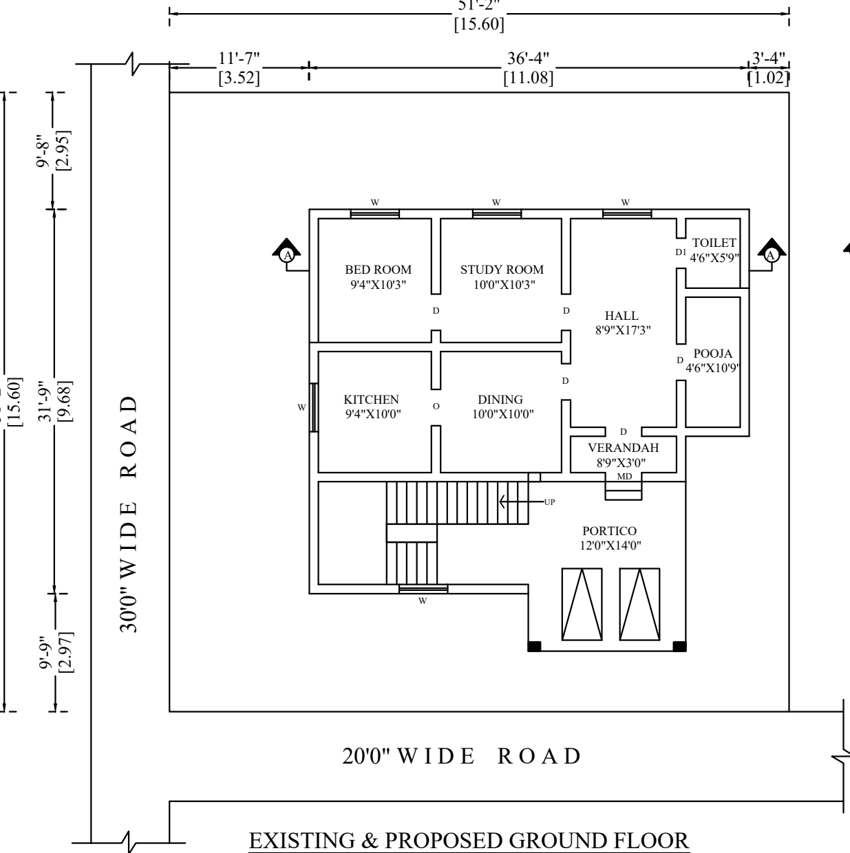
EXISTING & PROPOSED GROUND FLOOR
