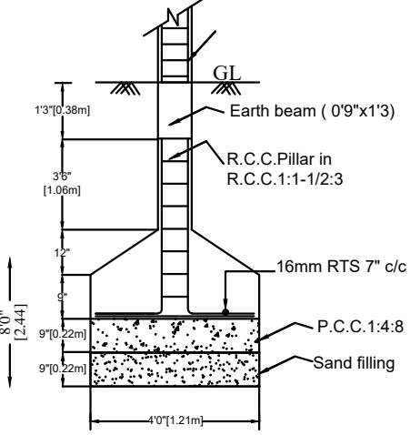
FOUNDATION DETAILS
