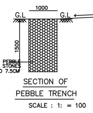
DETAILS OF SEPTIC TANK & DISPERSION TRENCH
