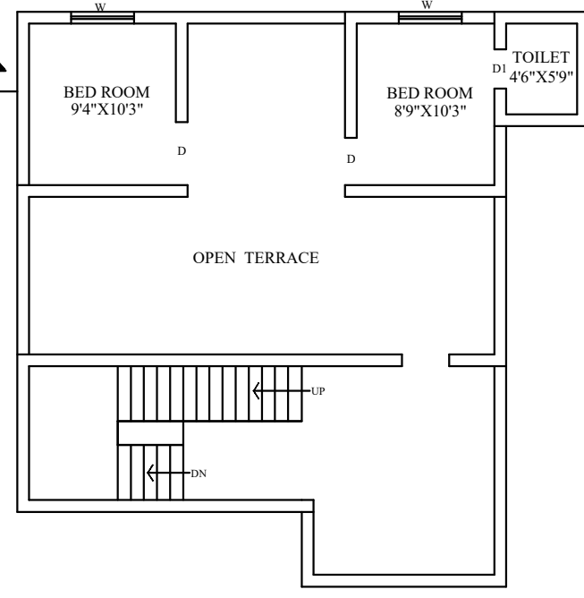
EXISTING & PROPOSED SECOND FLOOR
