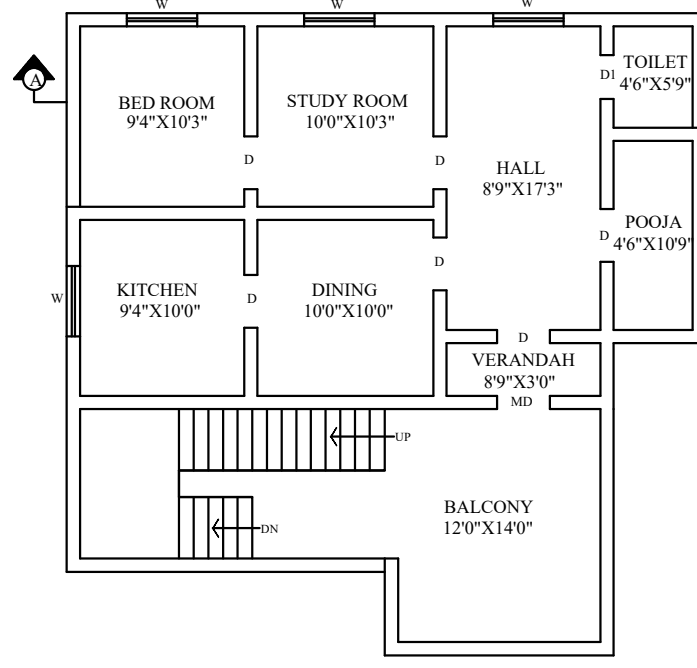
EXISTING & PROPOSED FIRST FLOOR
