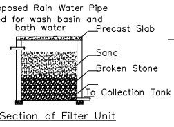
Section of Filter Unit
