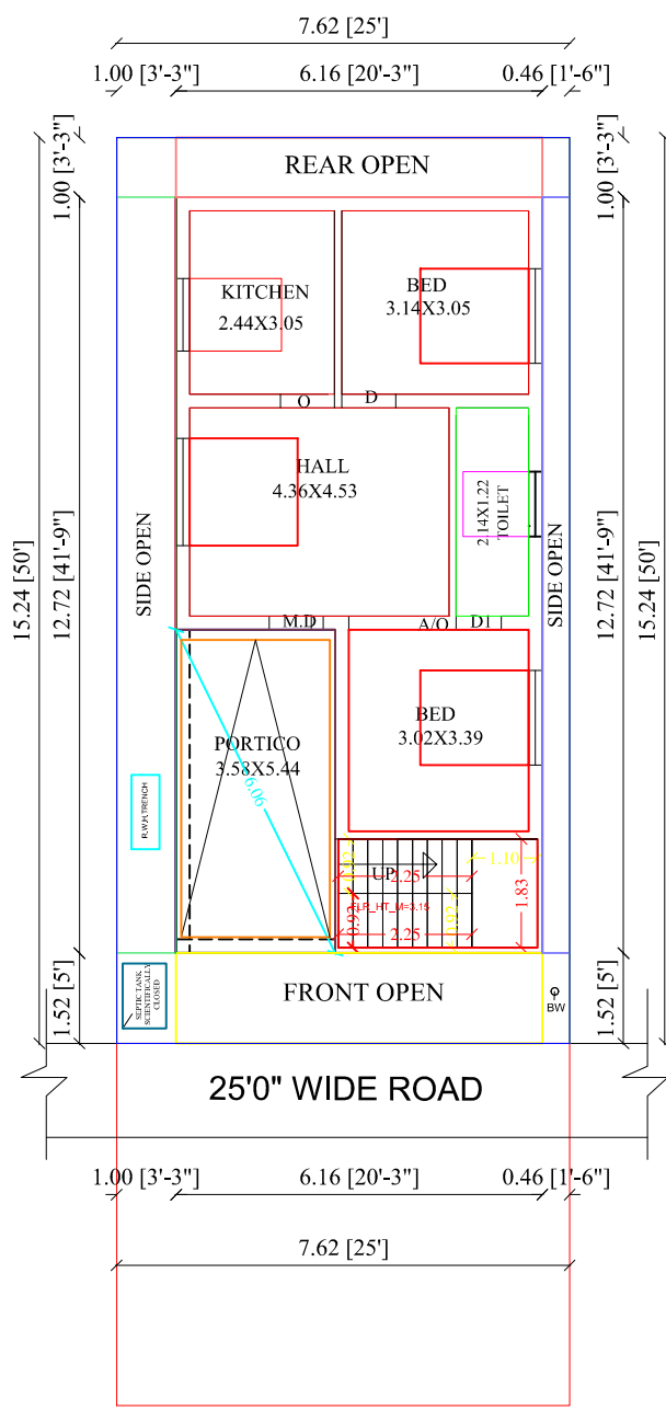
PRO.GROUND FLOOR PLAN
