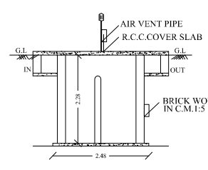
SEPTIC TANK DETAILS-SECTION
