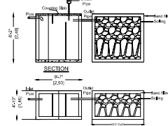
DETAILS OF SEPTIC TANK & DISPERSION TRENCH
