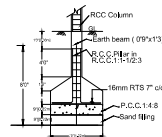
FOUNDATION DETAILS
