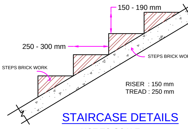
STAIRCASE DETAILS NOT TO SCALE
