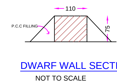
DWARF WALL SECTION NOT TO SCALE
