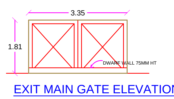
EXIT MAIN GATE ELEVATION
