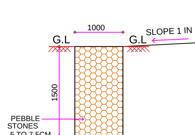
SECTION OF PEBBLE TRENCH SCALE : 1" = 100
