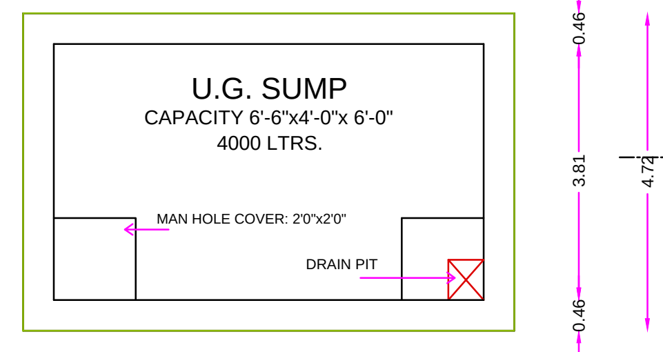
SUMP DETAIL SCALE 1"=2'-0"
