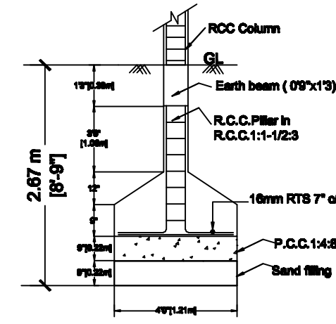
FOUNDATION DETAILS
