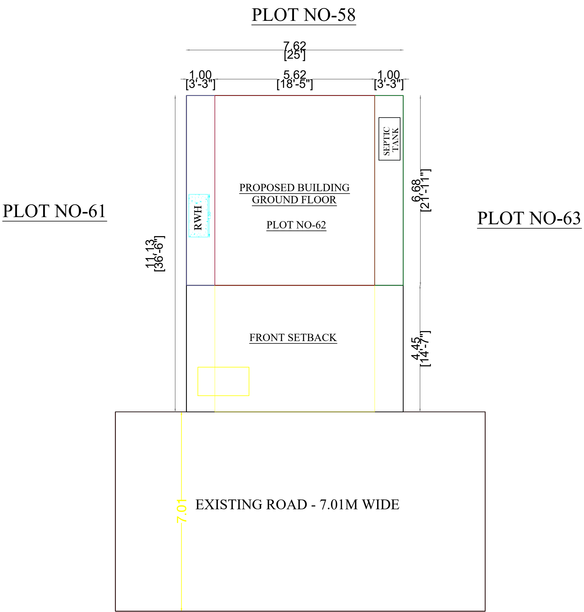
SITE PLAN
