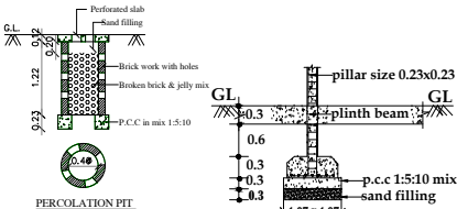
PERCOLATION PIT
