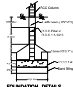
FOUNDATION DETAILS
