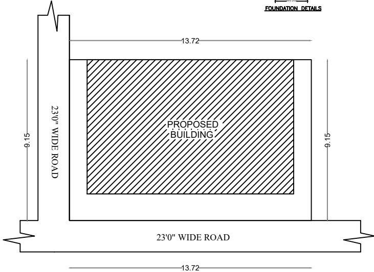
SITE PLAN
