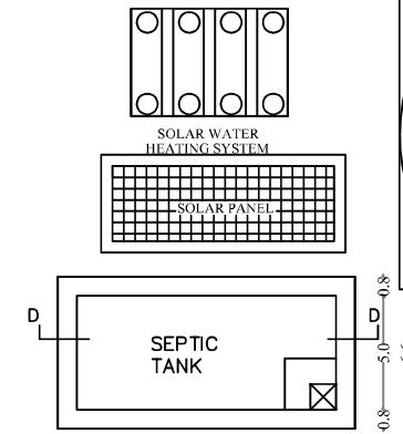
PLAN OF SEPTIC TANK SCALE 1"=2'0"
