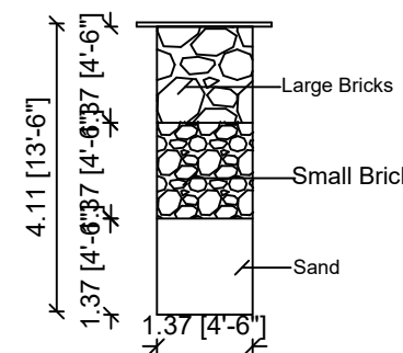
SECTION OF RAIN WATER
