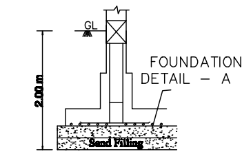
Isolated Footing -A (1.50X1.50) (Not to Scale)
