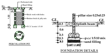
FOUNDATION DETAILS
