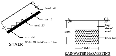
RAINWATER HARVESTING
