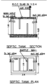
SEPTIC TANK PLAN
