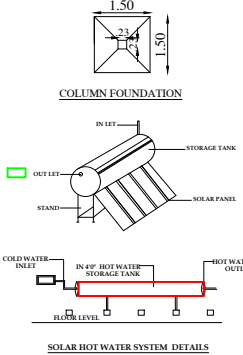
SOLAR HOT WATER SYSTEM DETAILS
