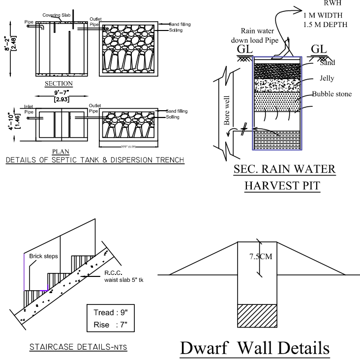
STAIRCASE DETAILS-NTS
