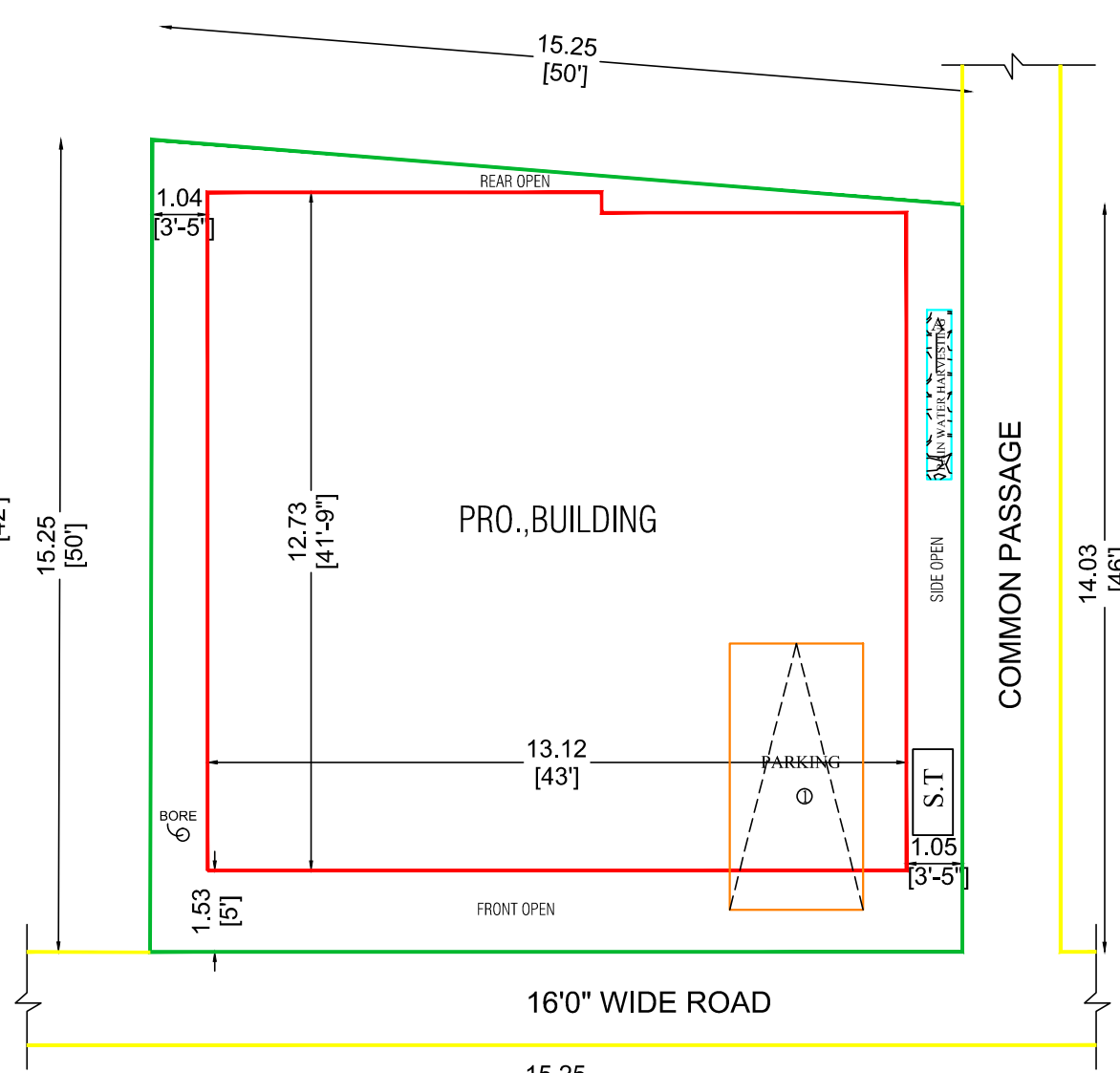
SITE PLAN
