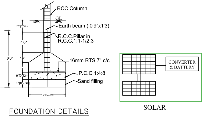
FOUNDATION DETAILS
