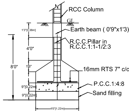
FOUNDATION DETAILS
