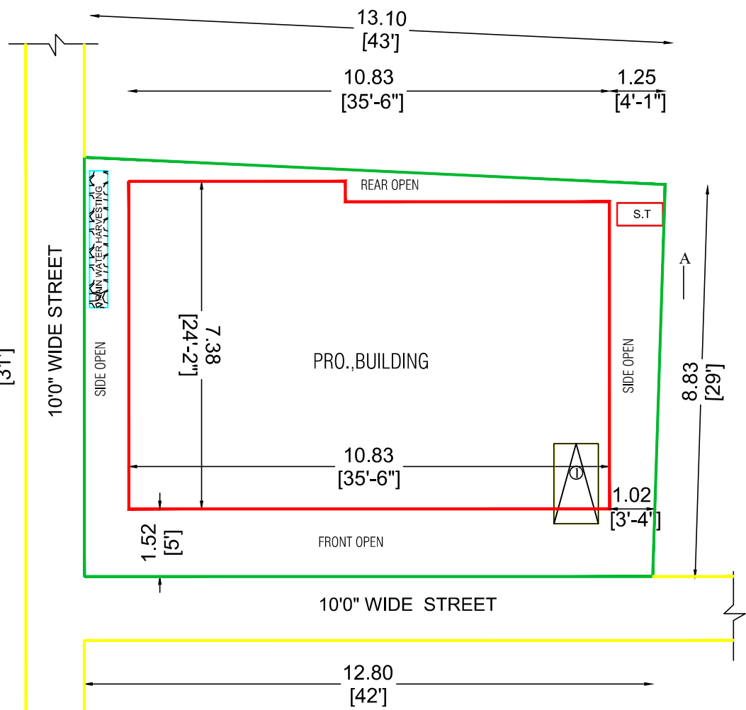
SITE PLAN
