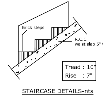
STAIRCASE DETAILS-nts
