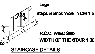
STAIRCASE DETAILS
