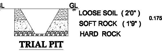
TRIAL PIT
