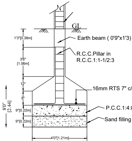
FOUNDATION DETAILS
