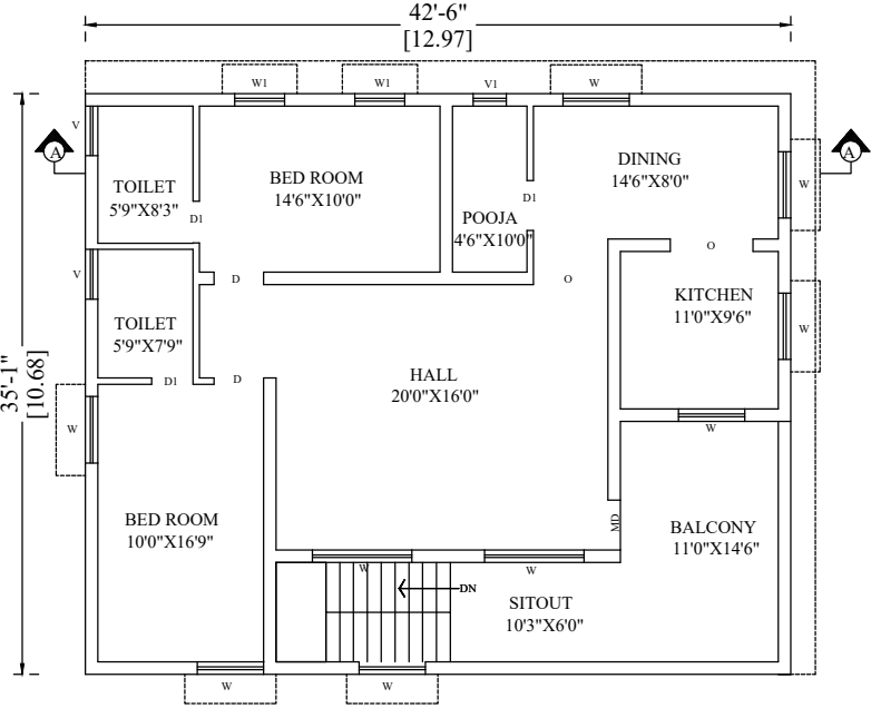
PROPOSED SECOND FLOOR
