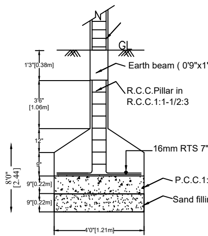
FOUNDATION DETAILS
