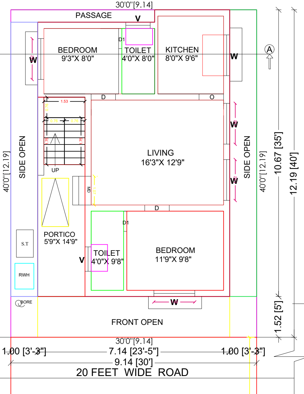
PRO.GROUND FLOOR PLAN
