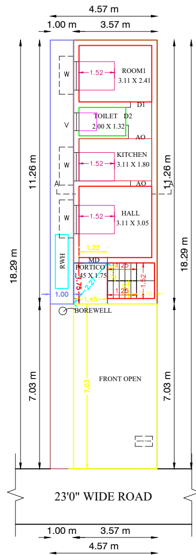
PRO. GROUND FLOOR PLAN
