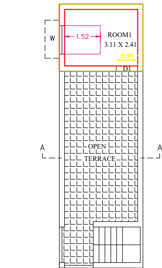
PRO. GROUND FLOOR PLAN
