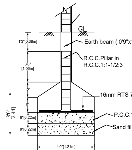
FOUNDATION DETAILS
