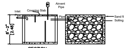
SECTION
