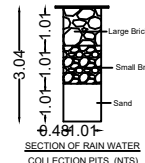
SECTION OF RAIN WATER COLLECTION PITS (NTS)
