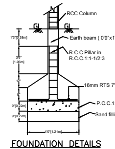
FOUNDATION DETAILS
