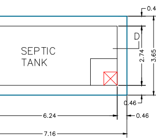
PLAN OF SEPTIC TANK SCALE 1"=2'0"
