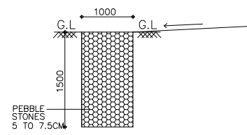
SECTION OF PEBBLE TRENCH SCALE : 1 : = 100
