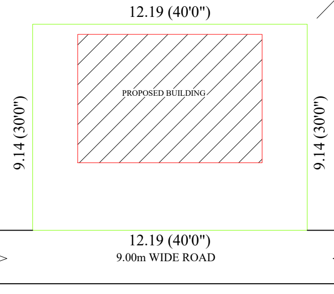
SITE PLAN
