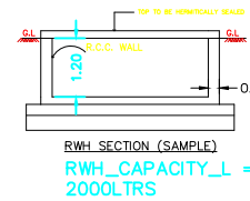
RWH_SECTION (SAMPLE) RWH_CAPACITY_L = 2000LTRS
