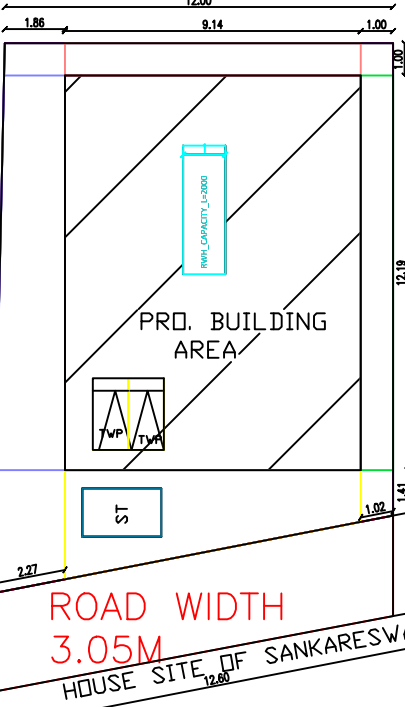
SITE PLAN
