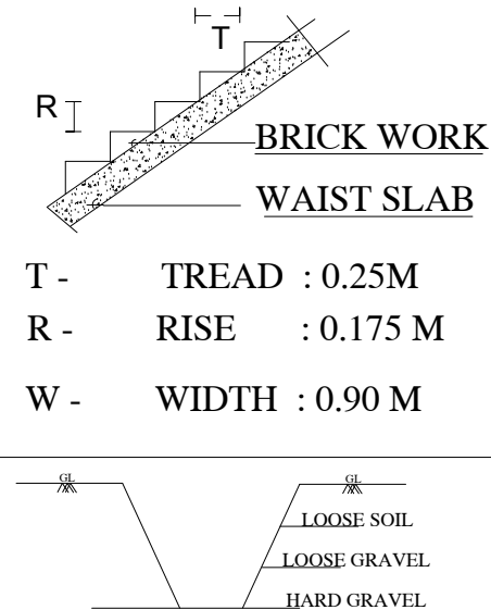
STAIRCASE DETAILS (NOT TO SCALE)
