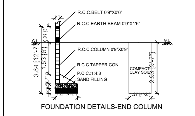
FOUNDATION DETAILS-END COLUMN
