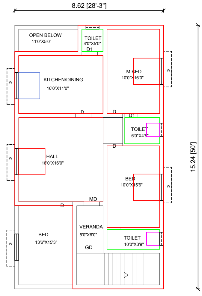
EXG.& PRO. FIRST FLOOR PLAN
