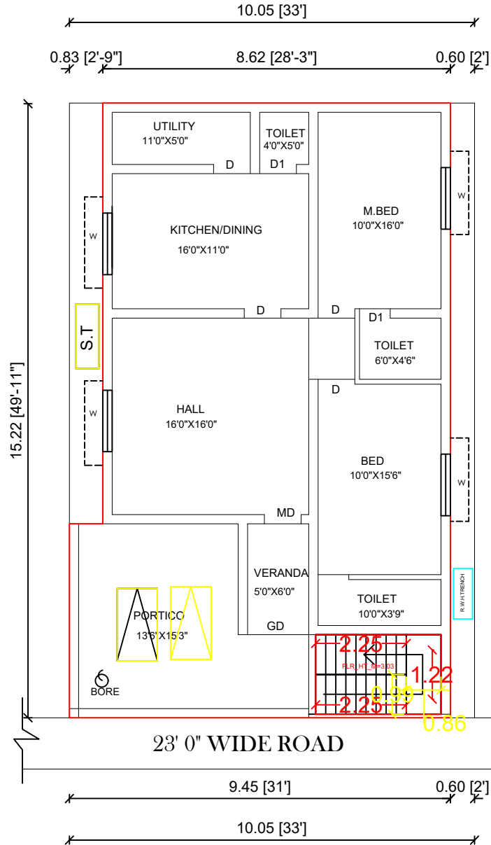
EXG .GROUND FLOOR PLAN
