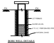
BORE WELL DETAILS
