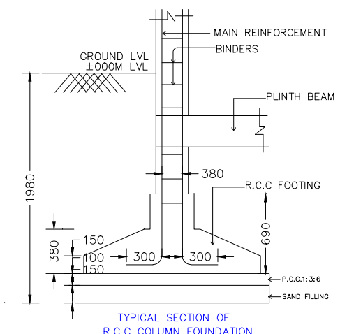
TYPICAL SECTION OF R.C.C. COLUMN FOUNDATION SCALE : 1" = 2'-0"
