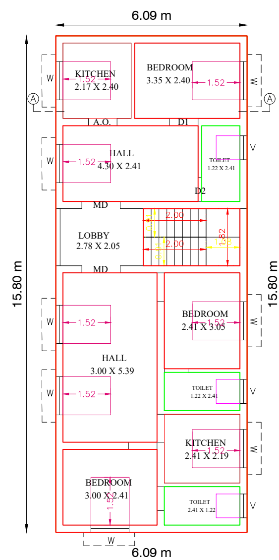
PRO.FIRST FLOOR PLAN
