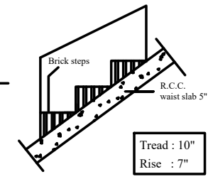
STAIRCASE DETAILS-nts
