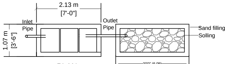
PLAN
