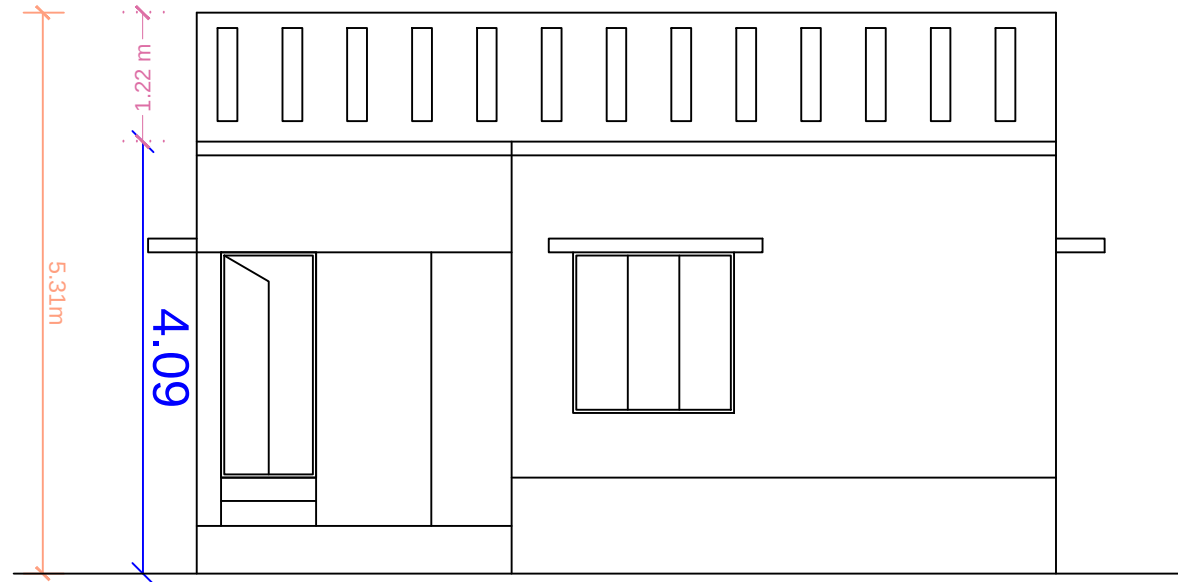
FRONT ELEVATION
