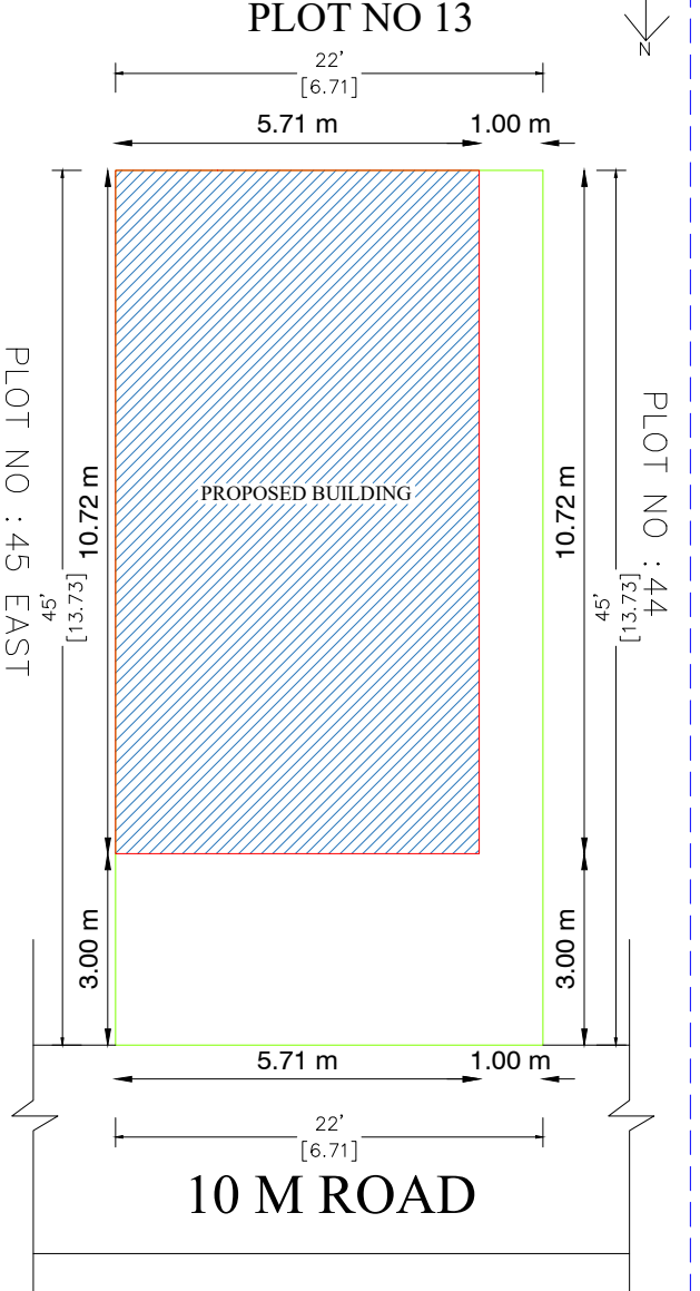
SITE PLAN
