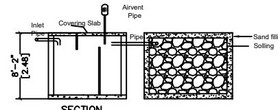
DETAILS OF SEPTIC TANK & DISPERSION TRENCH
