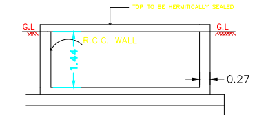
RWH SECTION (SAMPLE) RW_H_CAPACITY_L = 2000LTRS
