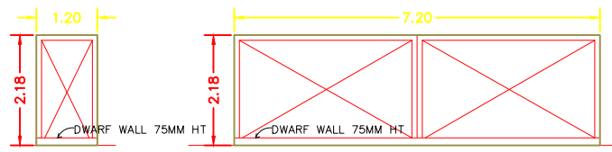
MAIN GATE
