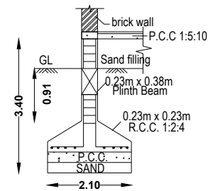
FOUNDATION DETAILS
