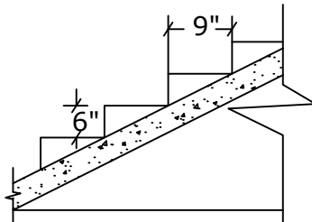
Staircase Detail Not To Scale
