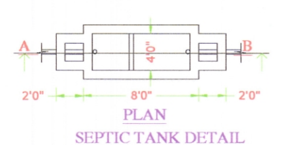
PLAN SEPTIC TANK DETAIL
